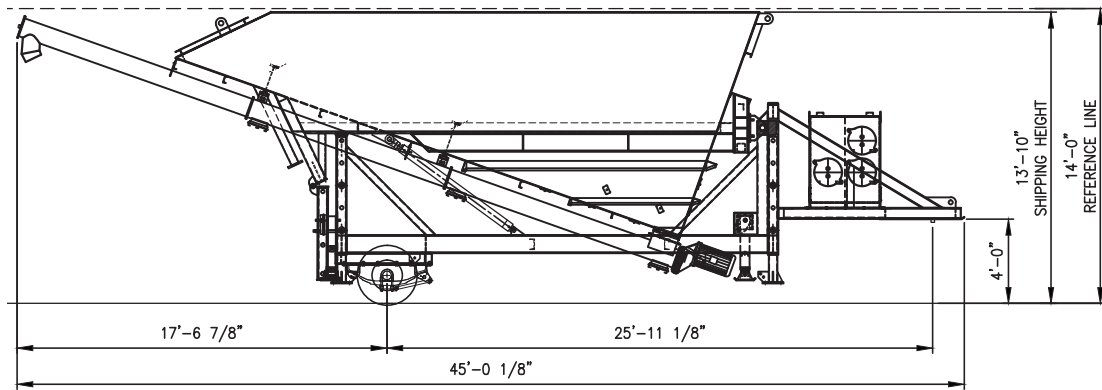
PONY EXPRESS: SHIPPING LAYOUT
